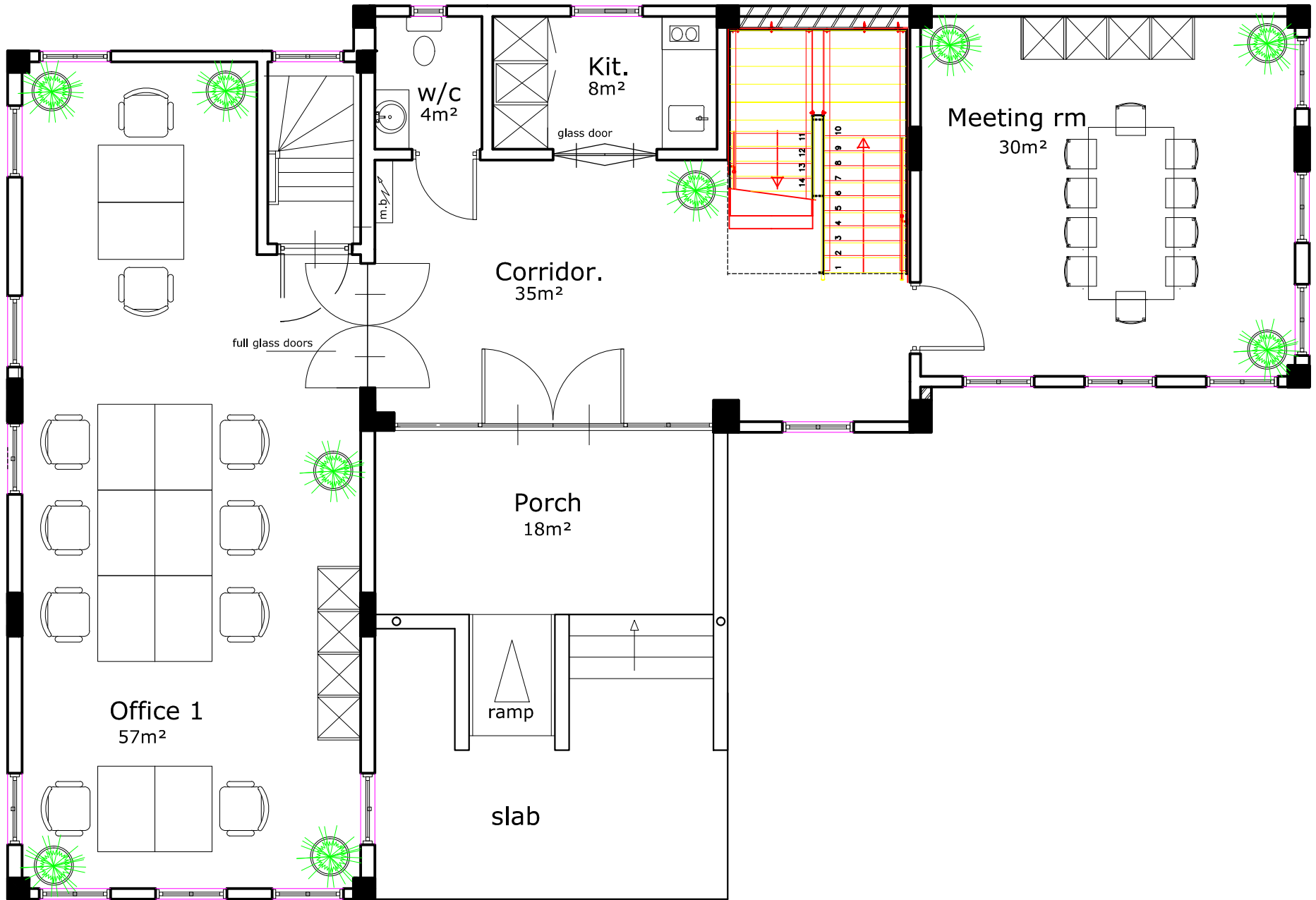
GROUND FLOOR NEW OFFICE (152m 2 )
